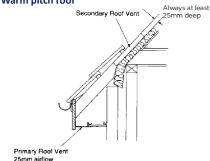
Fig. 3 Warm pitch roof
