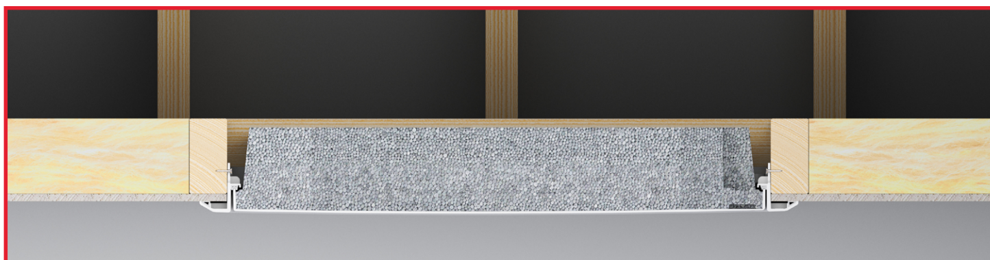
LT0025 | Fitted cross-section
