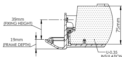
LT0035 | LT0035KL
