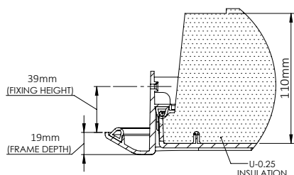
LT0025 | LT0025KL
