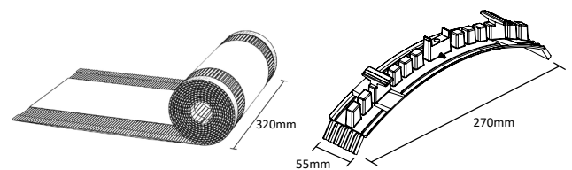
6m ridge roll
