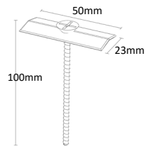
Screw, clamping plate & washer
