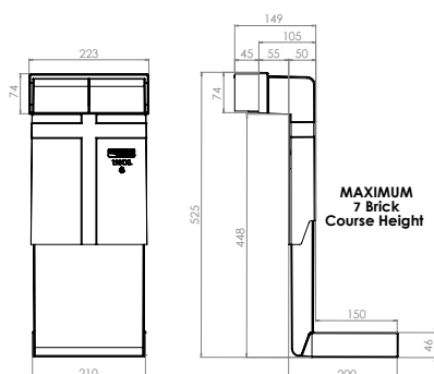
1201XL DIMENSIONS
