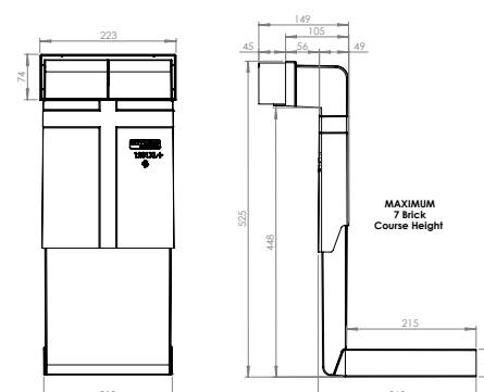
1201XL+ DIMENSIONS
