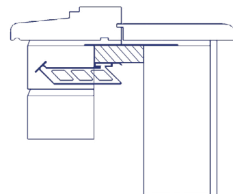
Sill detail
