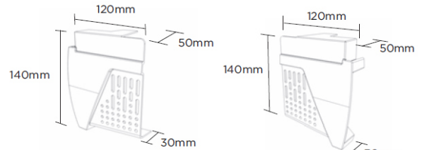
Dry fix verge eaves starter pack (right and left units)
