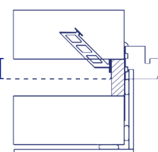
Staggered jamb
