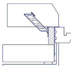
Fig. 2 Fully rebated (check reveal)
